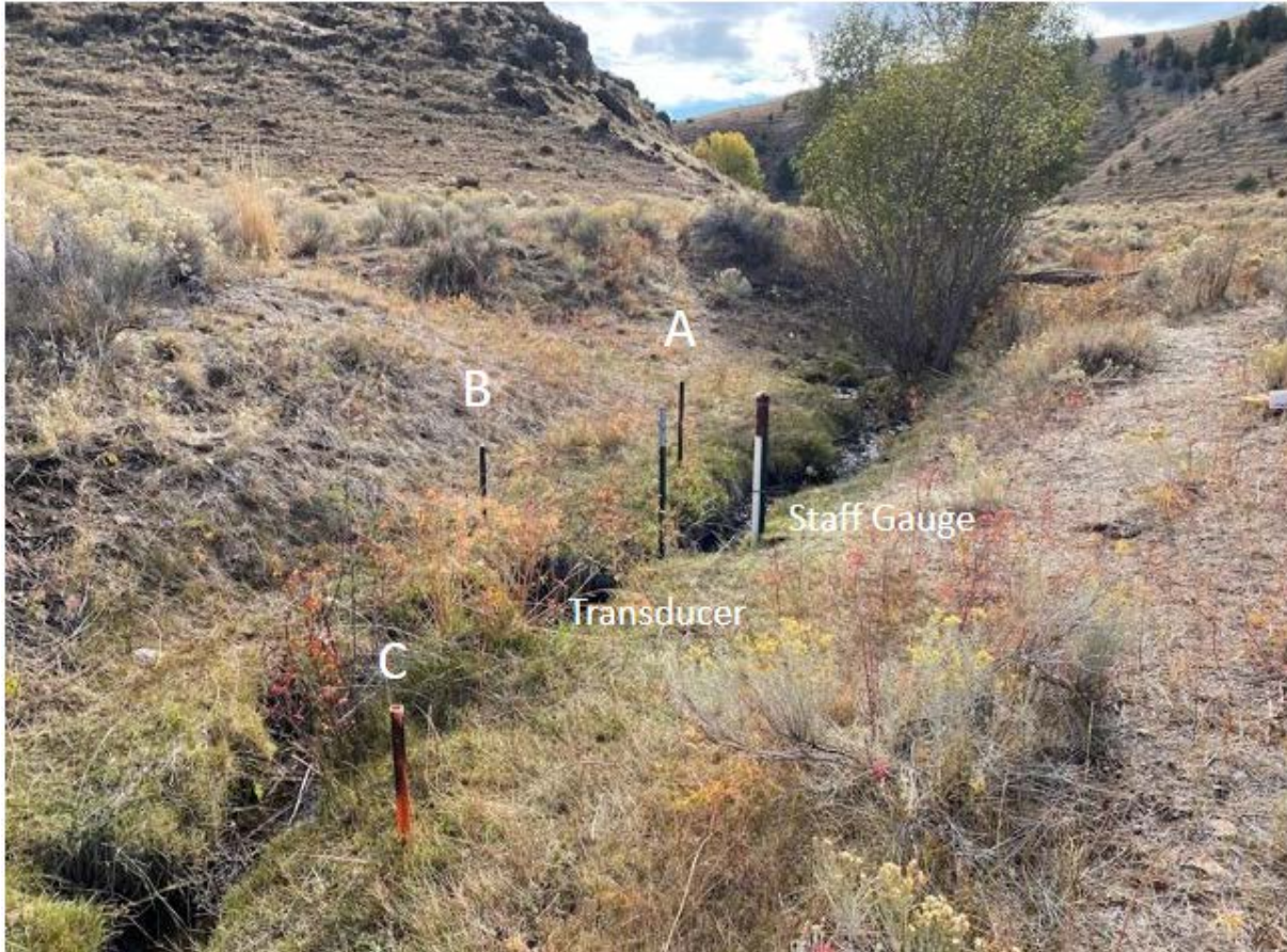
Figure 6: Groundwater monitoring site setup at Site 3. Wells at each site are labeled alphabetically from up to downstream.
