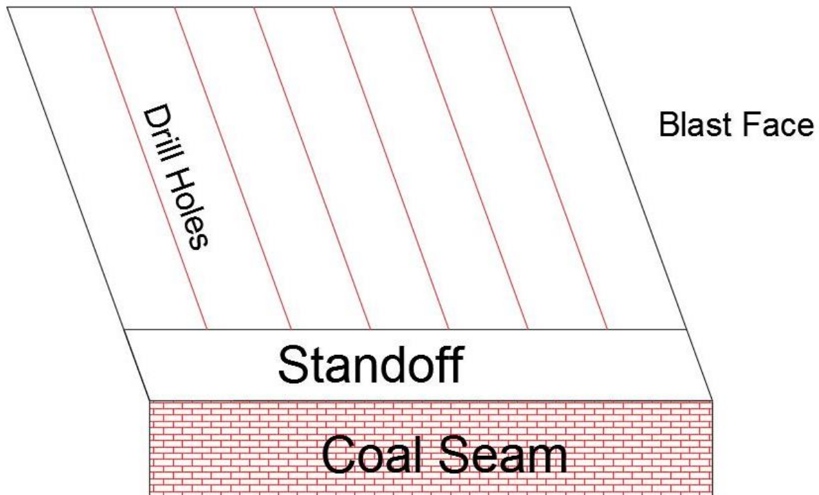
Figure 3: A cross-sectional concept drawing of how a traditional cast blast is drilled.
