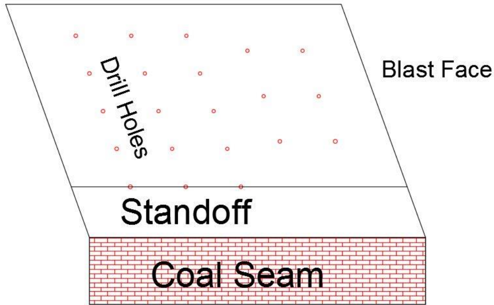
Figure 12: A cross-sectional concept drawing of how a hybrid cast blast is drilled.
