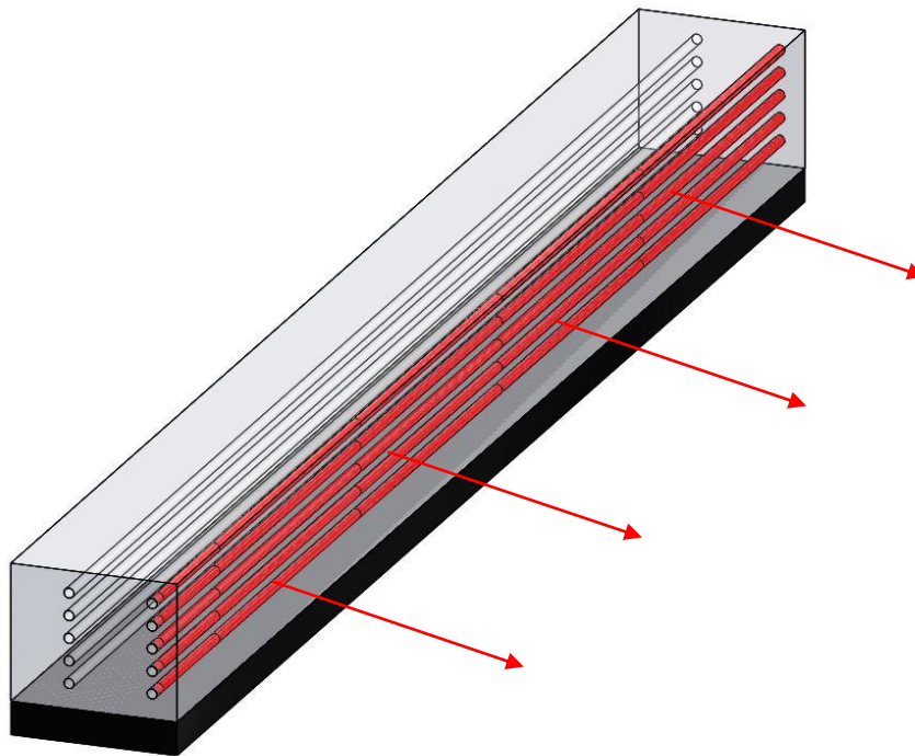
Figure 5: A 3-dimensional concept drawing of how the final drilled holes using directional drilling will be in relation to the blast face. The arrows represent the blast direction.
