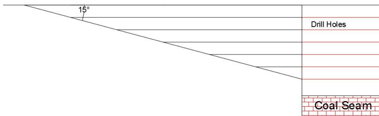
Figure 11: A directional cast blast pattern using a Ditch Witch drill rig.
