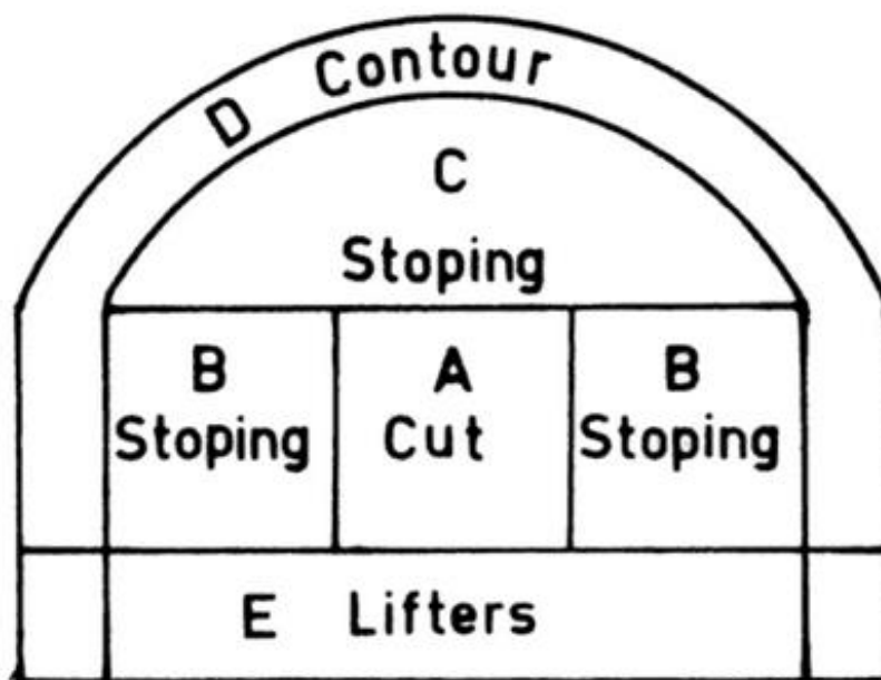
Figure 10: An underground blast face. Sections A-E represent holes with different blasting conditions. (Persson, 1964, p. 219)
