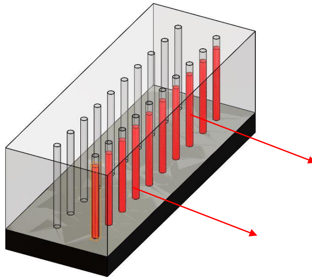
Figure 2: A 3-dimensional concept drawing of how a traditional cast blast is drilled and the relation of the drill holes to the blast face. The arrows represent the blasted material movement direction.
