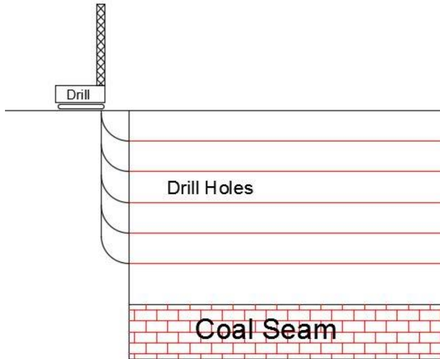
Figure 6: A cross-sectional concept drawing of how a cast blast is drilled using directional drilling.
