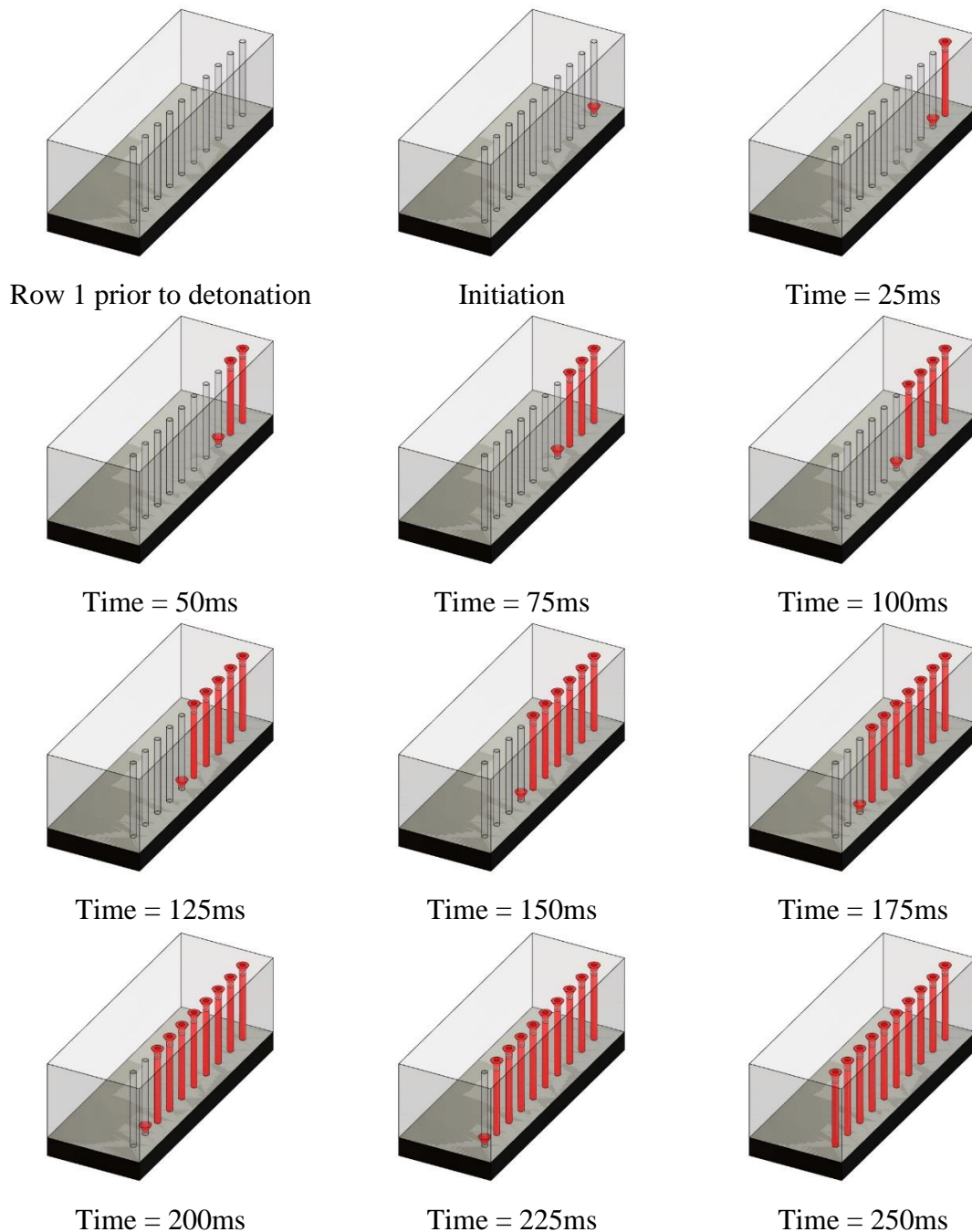
Figure 4: This series of figures shows a general timing sequence for a traditional cast blast. It should be noted that this timing sequence produces a peeling affect as mentioned above.
